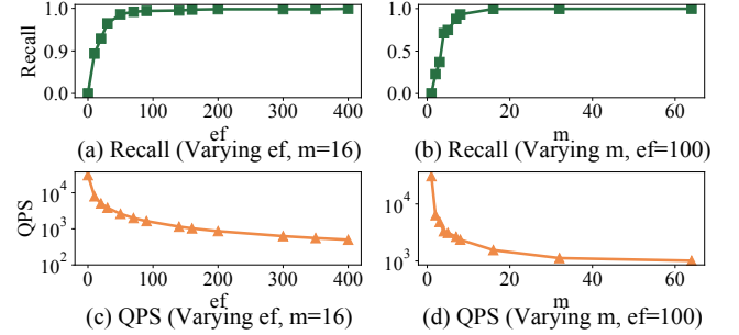
Figure 13: Performance on different search parameters.
