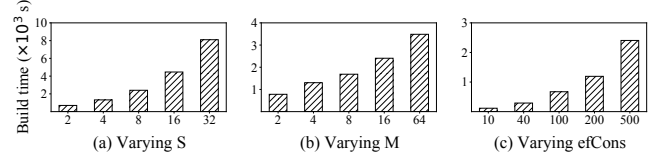
Figure 12: Index build time on different index parameters.
