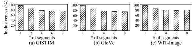
Figure 7: Inclusiveness of HSIG.
