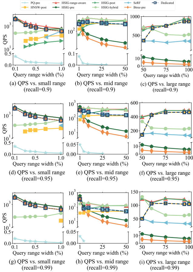
Figure 6: Impact of different query ranges on GloVe dataset.
