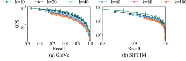
Figure 14: Performance of different k values.
