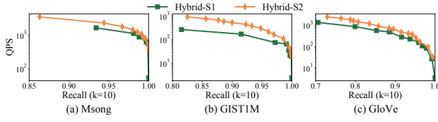
Figure 10: Impact of the runtime neighbor selection method.
