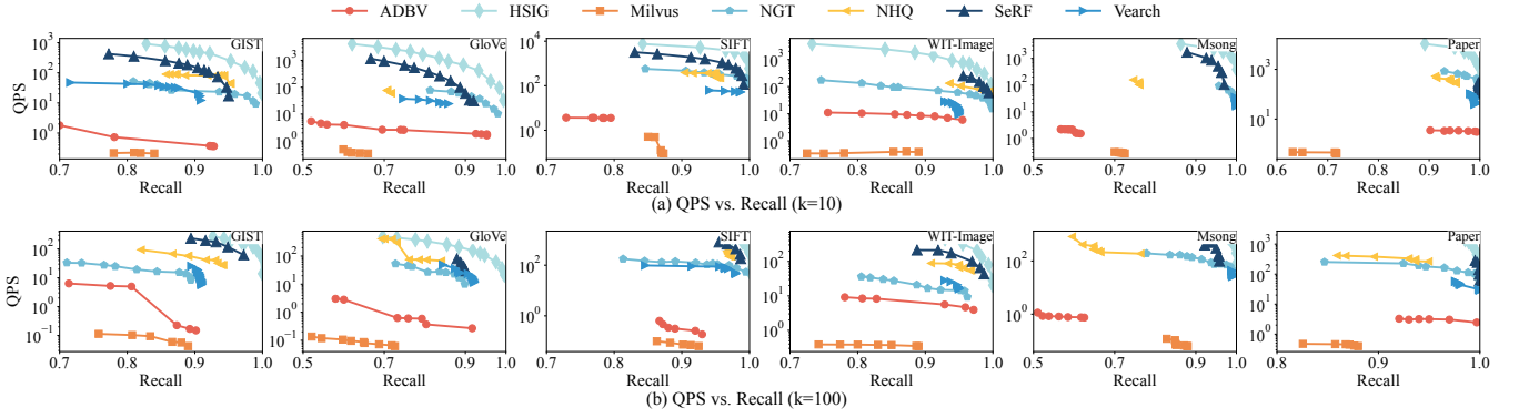
Figure 5: Overall Performance.
