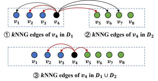
Figure 1: Build multiple k NNGs exhaustively ( k = 3 ).
