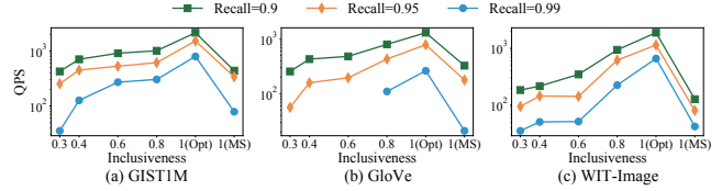
Figure 8: Impact of Inclusivity.
